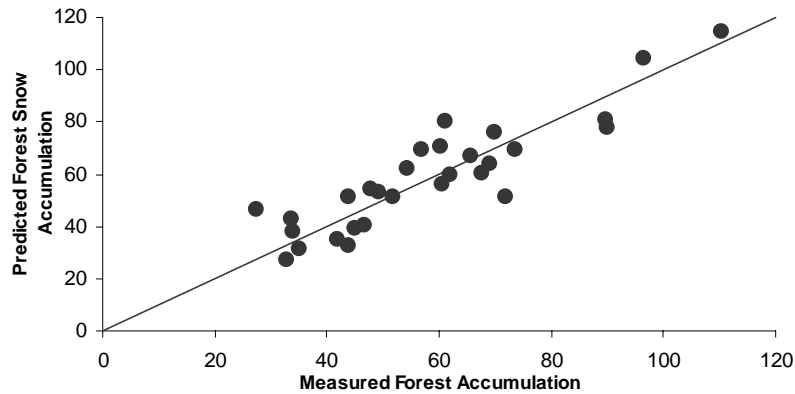
Fig. 2 Points indicating measured seasonal forest snow accumulation (mm) and that predicted using equation (9) using snowfall event size, p_c , of 5 mm and sublimation efficiency, e_s , of 0.72 and a 1:1 line for reference.
