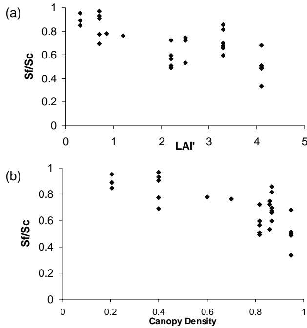
Fig. 1 Ratio of forest to clearing snow accumulation as a function of stand characteristics: (a) leaf area index (effective winter), (b) canopy density (winter).
