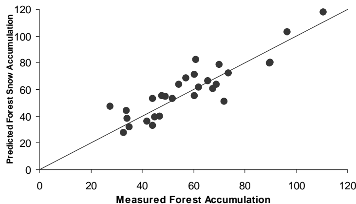
Fig. 3 Performance of the parametric forest snow accumulation equation (equation (9)) presuming that sublimation efficiency is 0.72; measured and modelled accumulation (mm) as points with a 1:1 line for comparison.
